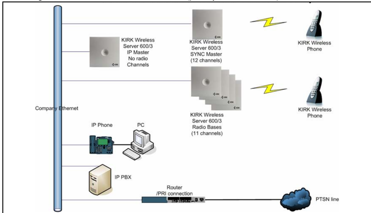
Figure 94 KWS600v3 Multi-cell installation (primary and secondaries)
